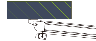
Articulated Roof Fixation Piece 铰接式屋顶固定件
