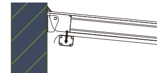
Articulated Wall Fixation Piece 铰接式墙固定件
