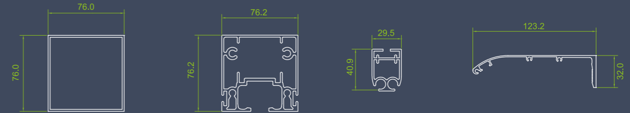
Measure of Pillars 铝材尺寸
