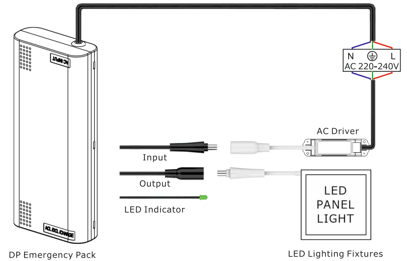
Wiring Diagram of DP Emergency Pack
